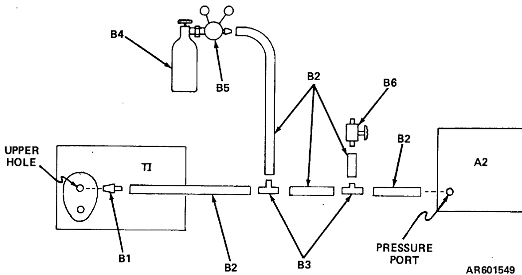
Figure 4. Resistance gage performance check, equipment setup.
